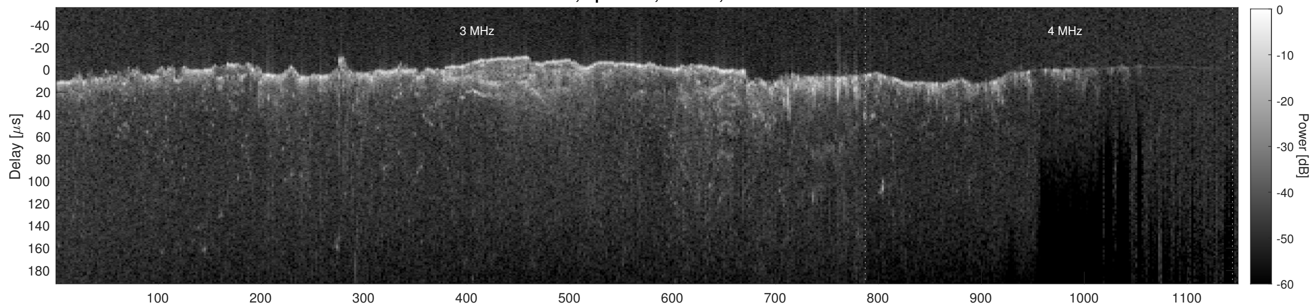
Orbit 12878, Cluttergram
