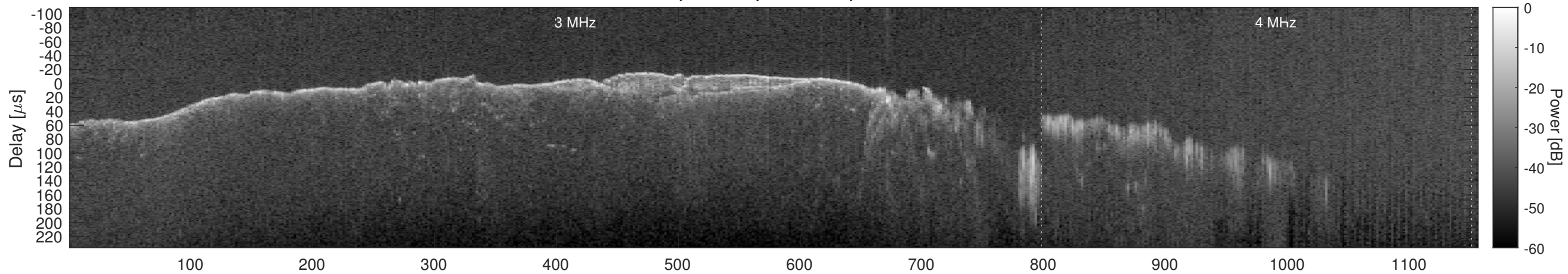
Orbit 12882, Window, Channel 2, Chapman
