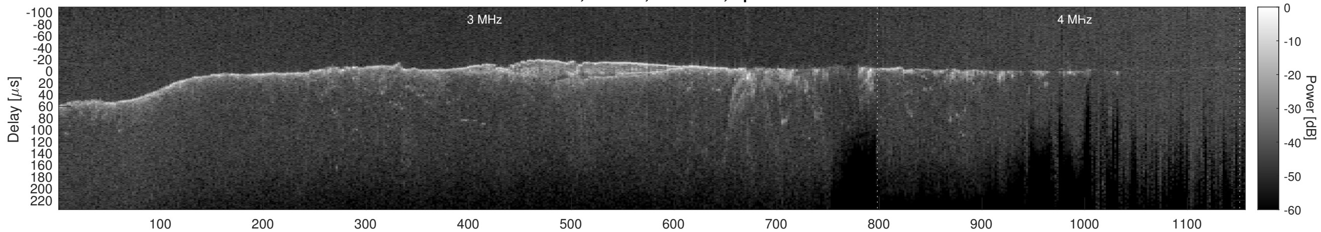
Orbit 12882, Cluttergram
