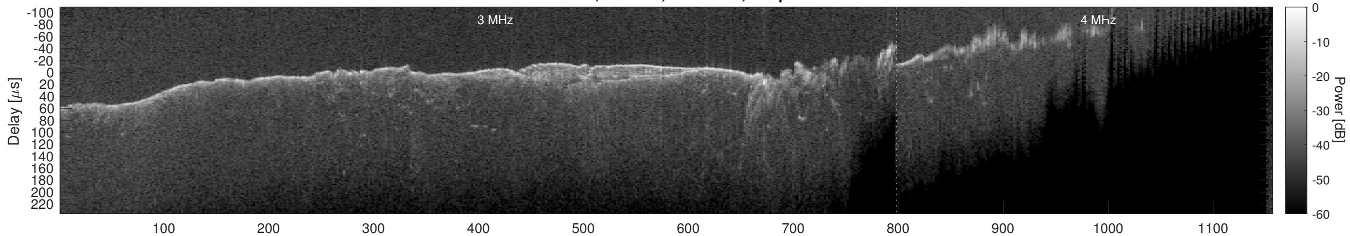
Orbit 12882, Window, Channel 2, Optimized
