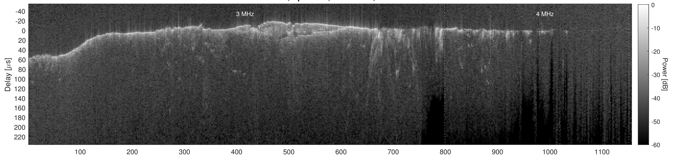
Orbit 12882, Cluttergram
