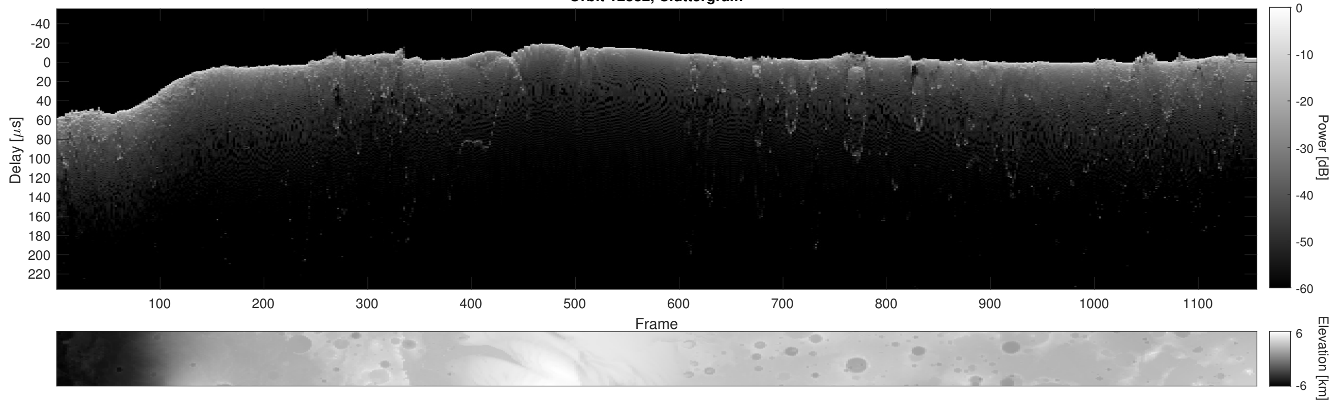
Orbit 12882, Cluttergram
