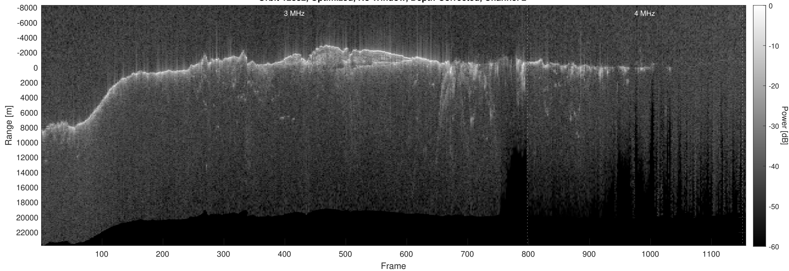
Orbit 12882, Optimized, No Window, Depth-Corrected, Channel 2
