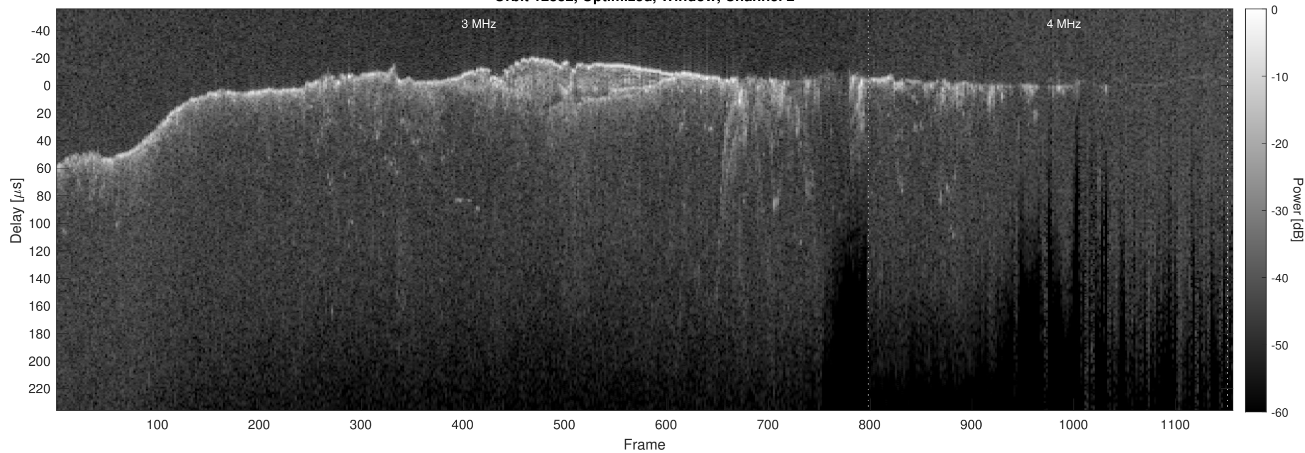
Orbit 12882, Optimized, Window, Channel 2
