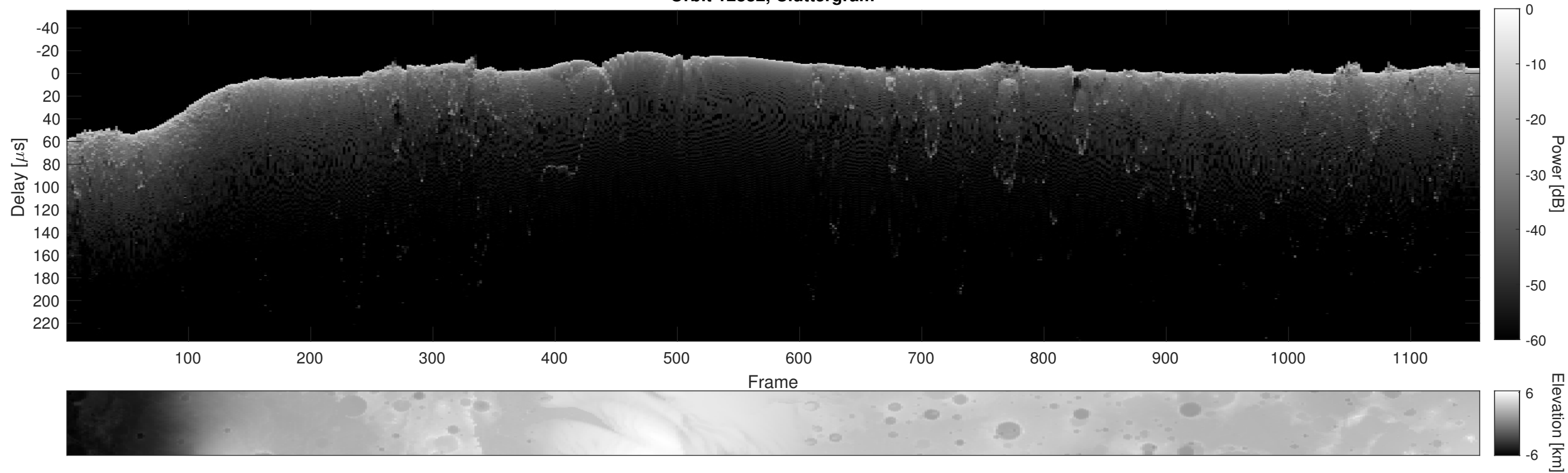
Orbit 12882, Cluttergram
