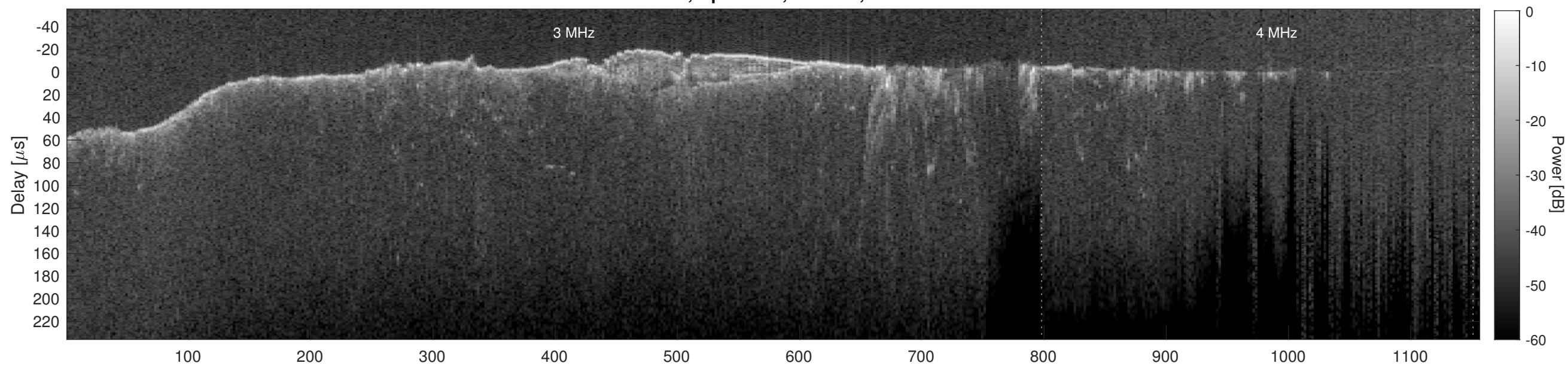
Orbit 12882, Cluttergram
