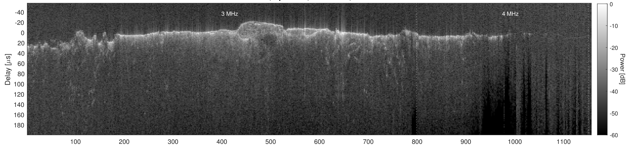
Orbit 12883, Cluttergram
