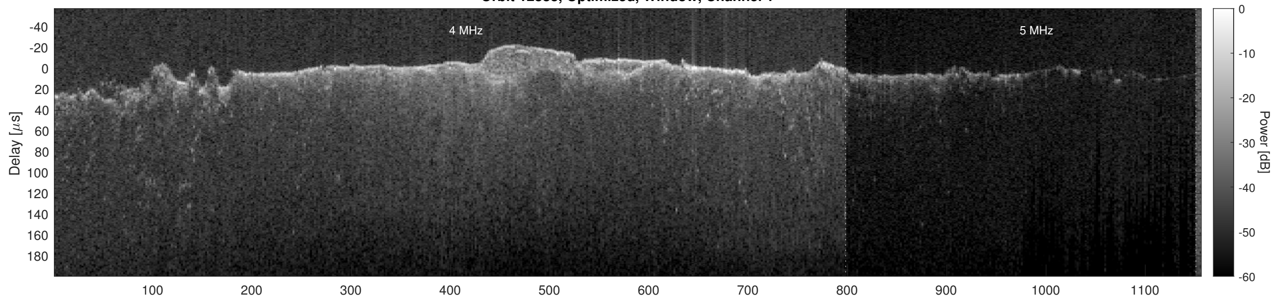
Orbit 12883, Optimized, Window, Channel 2
