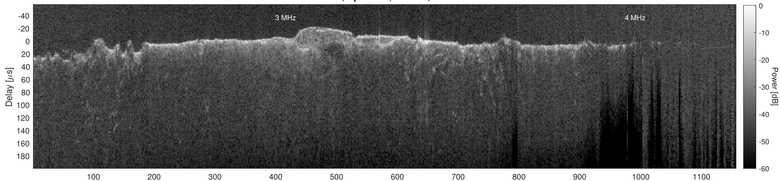
Orbit 12883, Cluttergram
