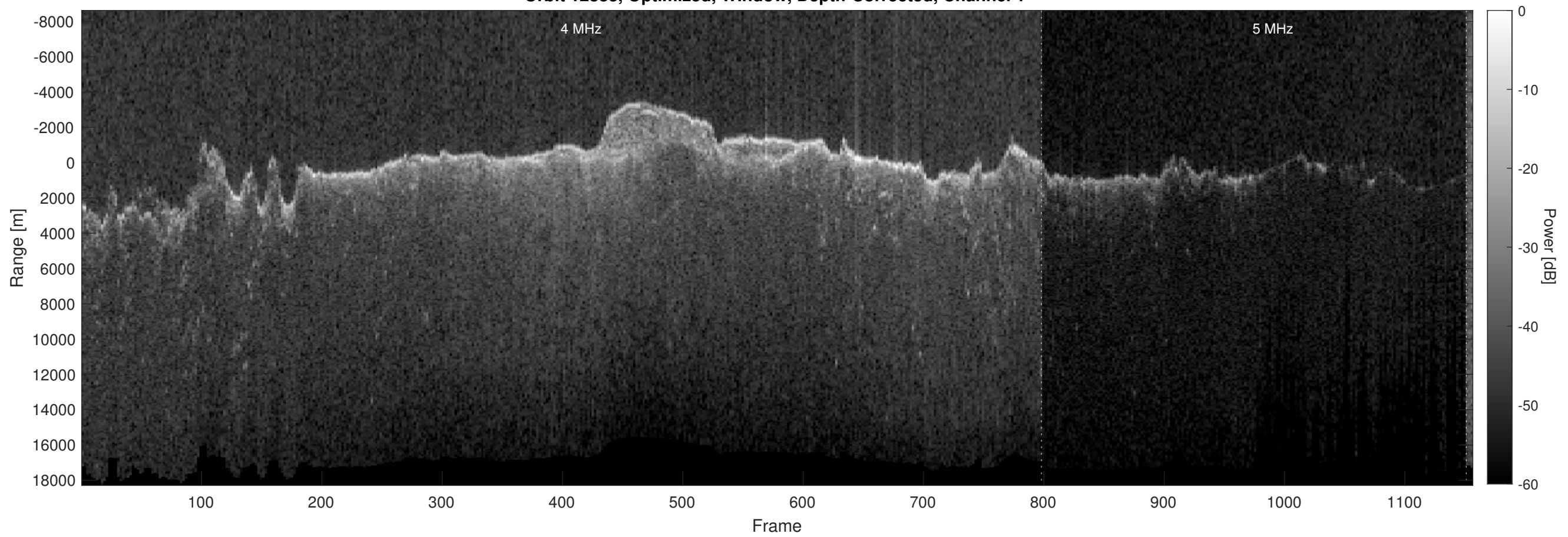
Orbit 12883, Optimized, Window, Depth-Corrected, Channel 2
