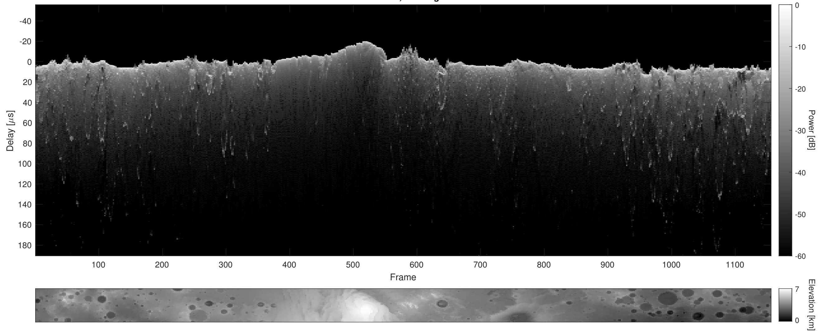
Orbit 12884, Cluttergram
