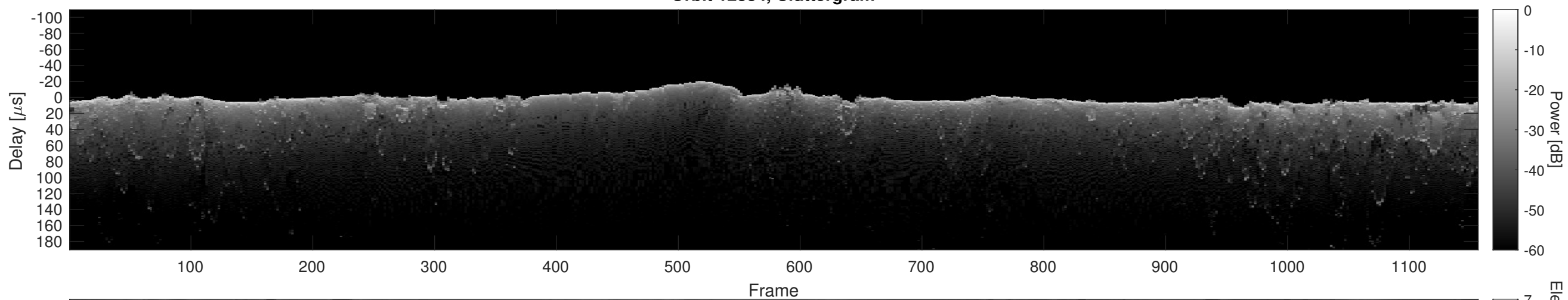
Orbit 12884, Cluttergram
