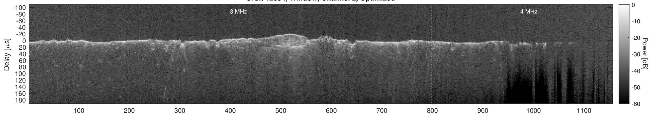
Orbit 12884, Cluttergram
