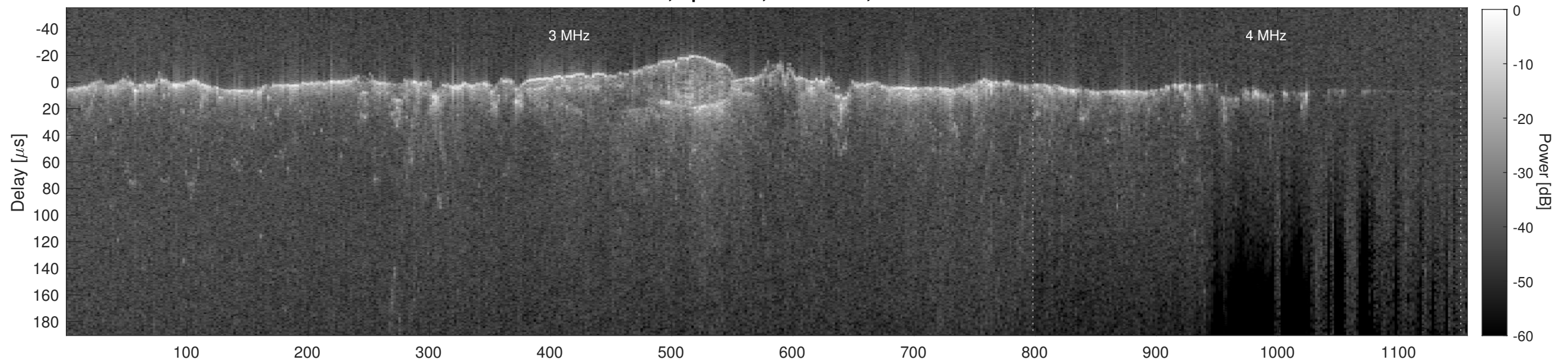
Orbit 12884, Cluttergram
