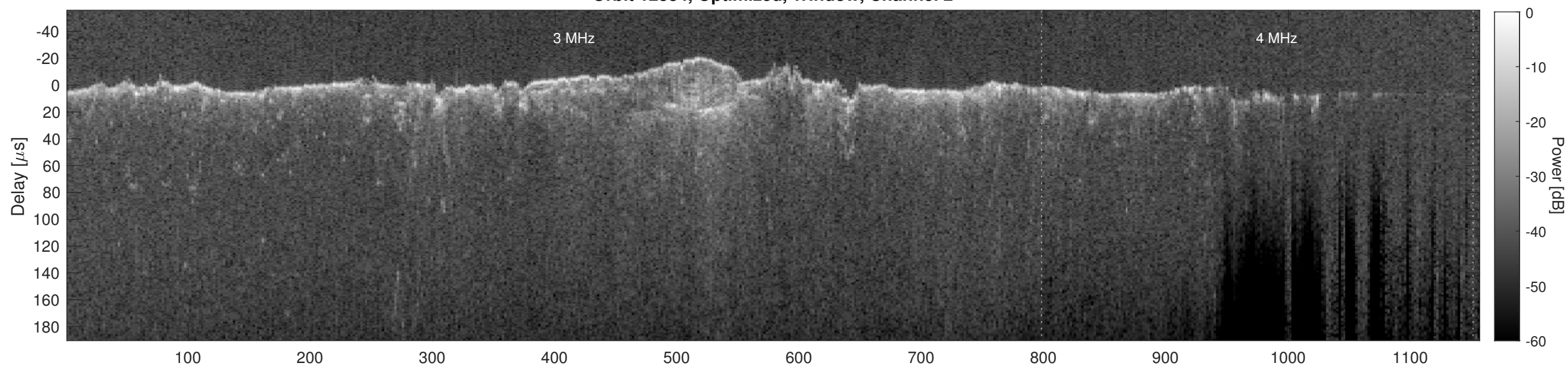
Orbit 12884, Cluttergram
