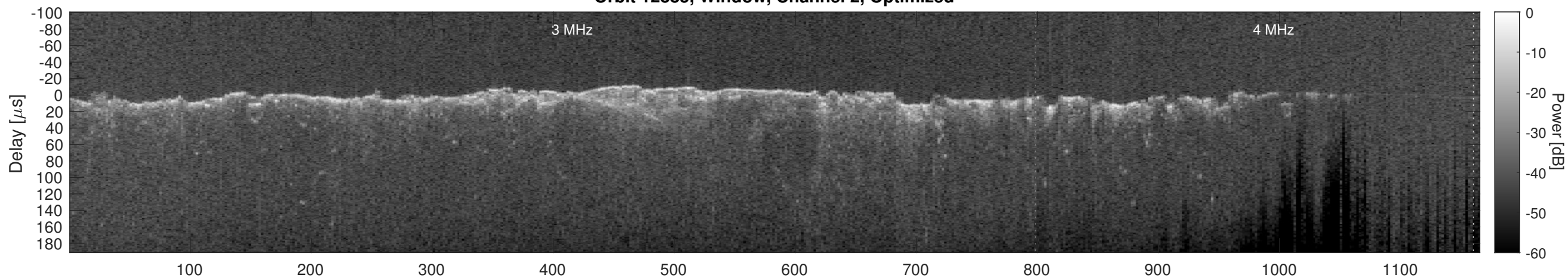
Orbit 12885, Cluttergram
