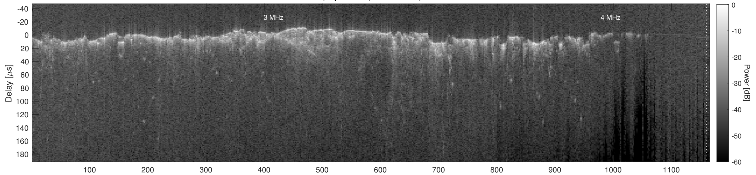
Orbit 12885, Cluttergram
