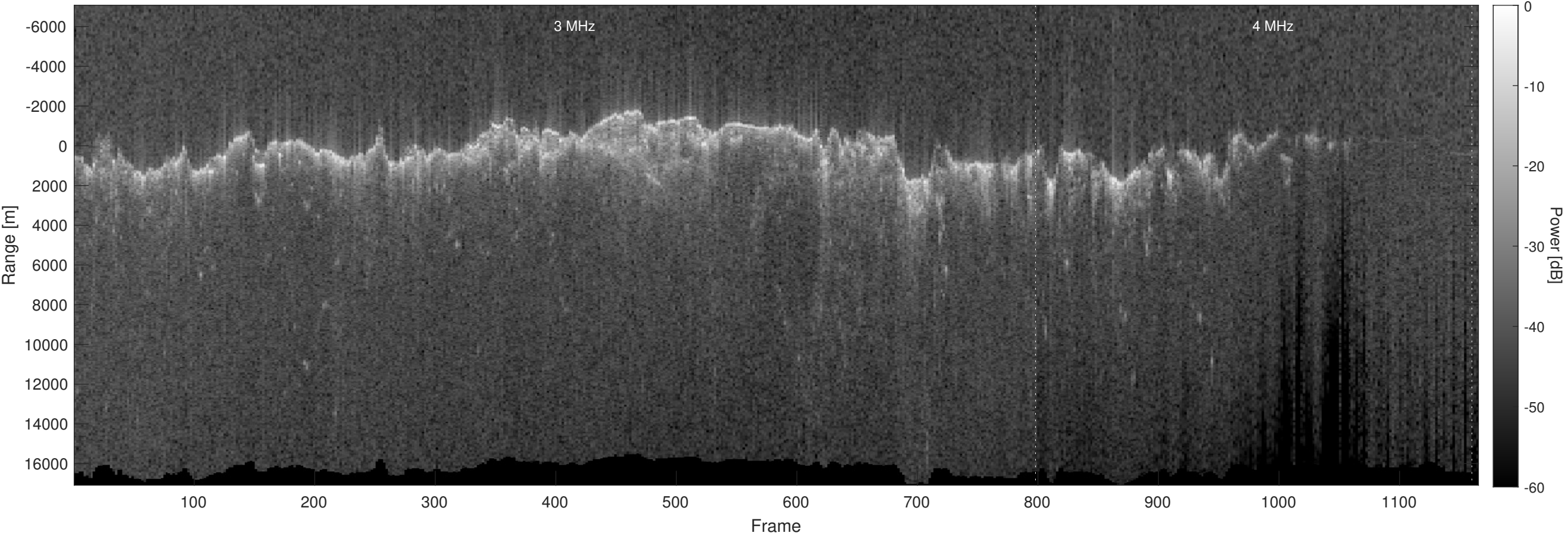
Orbit 12885, Optimized, No Window, Depth-Corrected, Channel 2
