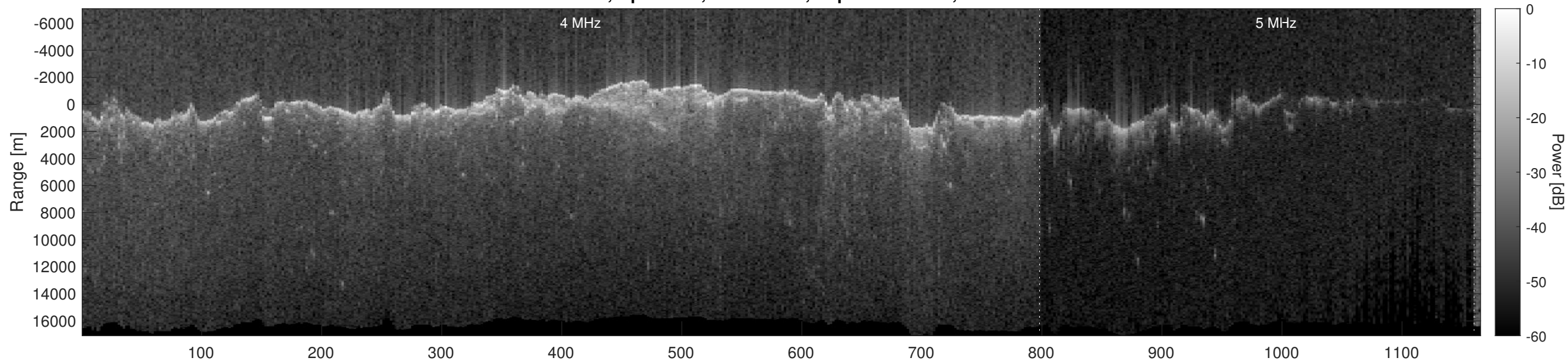
Orbit 12885, Optimized, No Window, Depth-Corrected, Channel 2
