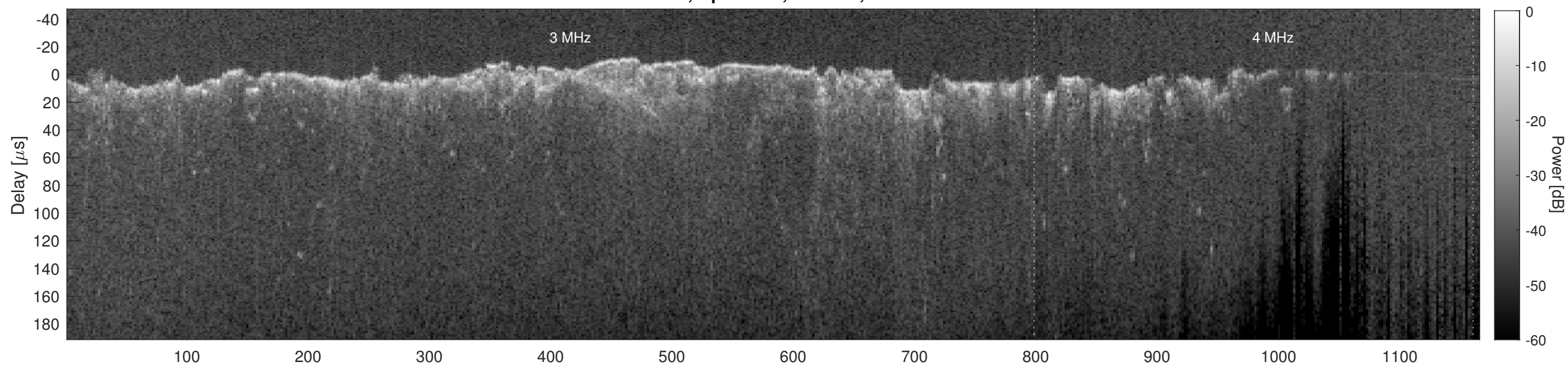
Orbit 12885, Cluttergram
