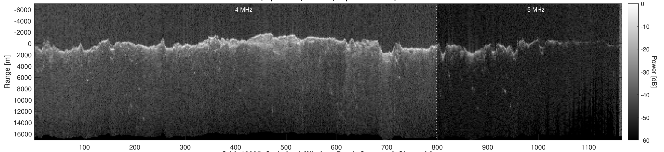
Orbit 12885, Optimized, Window, Depth-Corrected, Channel 2
