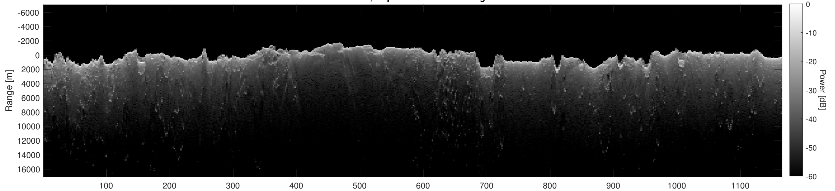
Orbit 12885, Depth-Corrected Cluttergram
