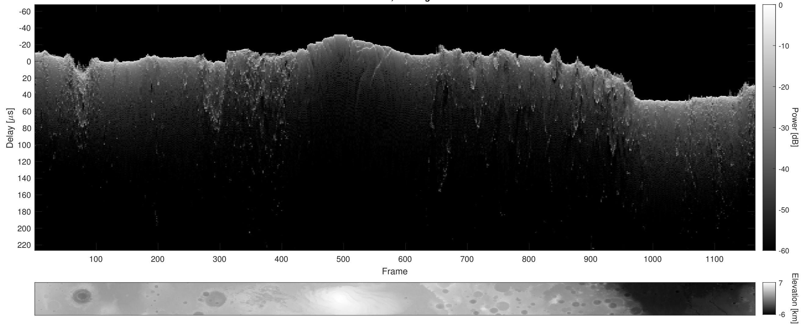
Orbit 12887, Cluttergram
