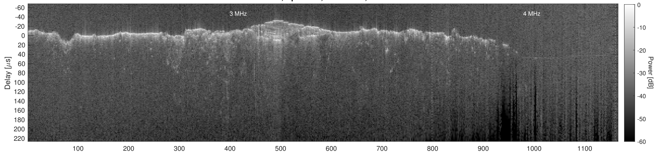
Orbit 12887, Cluttergram
