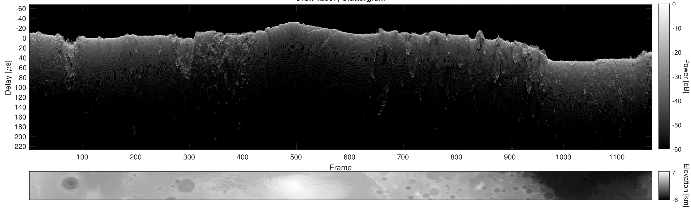
Orbit 12887, Cluttergram
