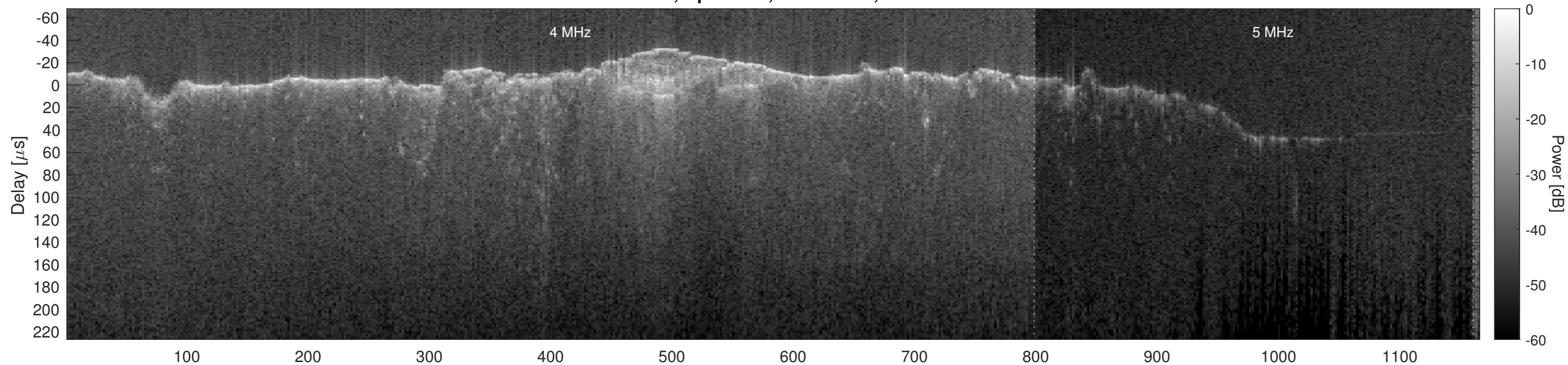
Orbit 12887, Optimized, No Window, Channel 2
