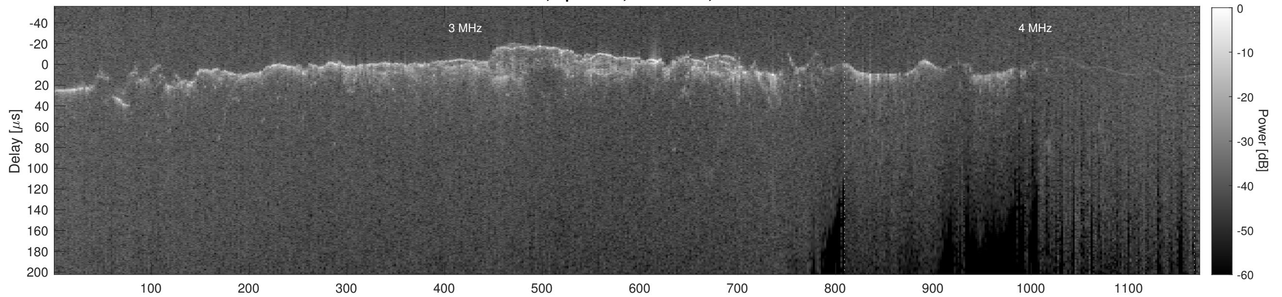
Orbit 12890, Cluttergram
