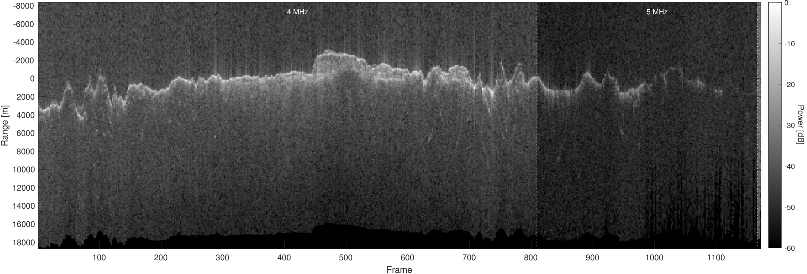
Orbit 12890, Optimized, No Window, Depth-Corrected, Channel 2
