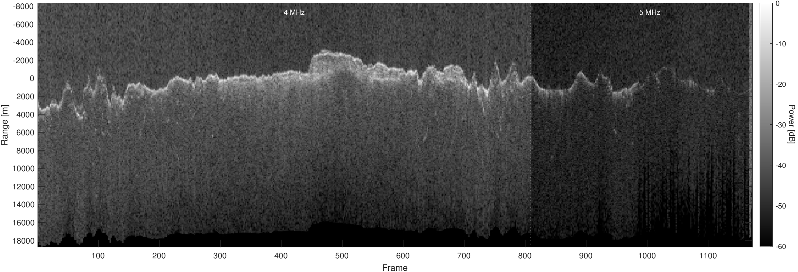
Orbit 12890, Optimized, Window, Depth-Corrected, Channel 2
