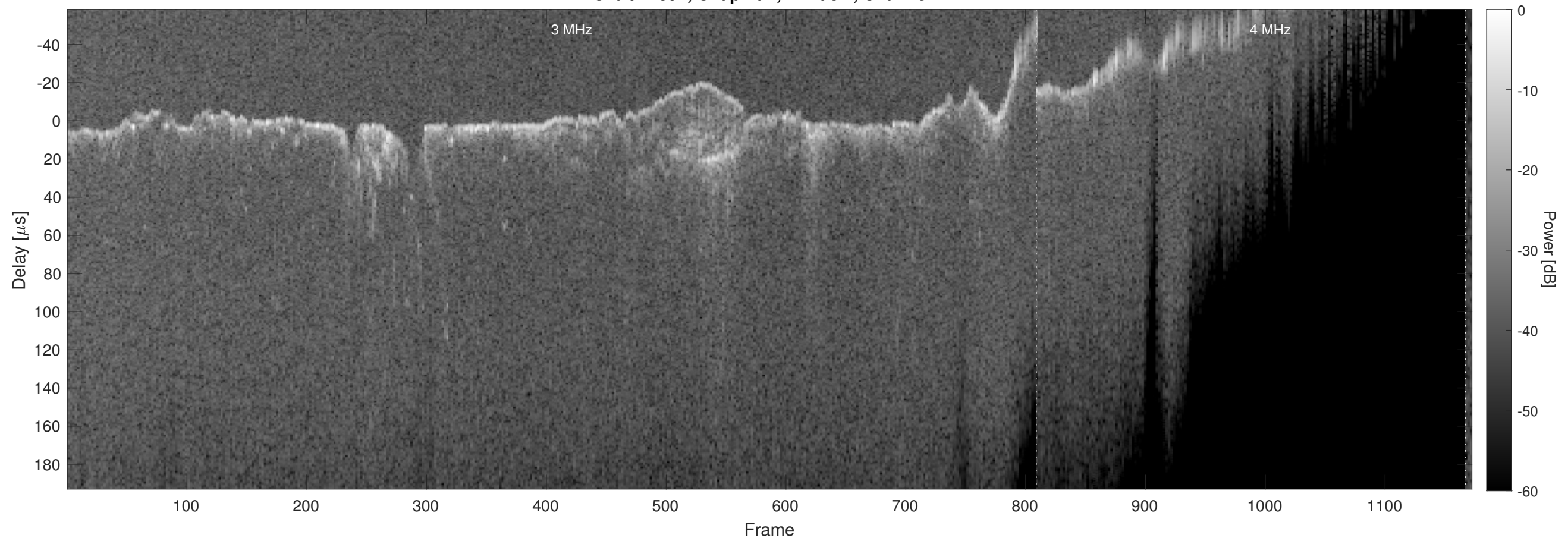
Orbit 12891, Chapman, Window, Channel 2
