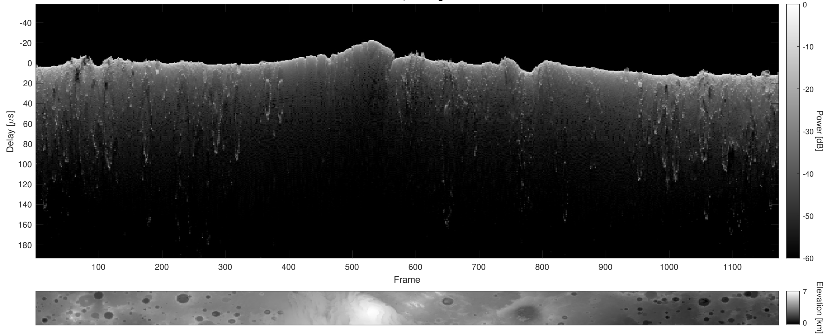
Orbit 12891, Cluttergram
