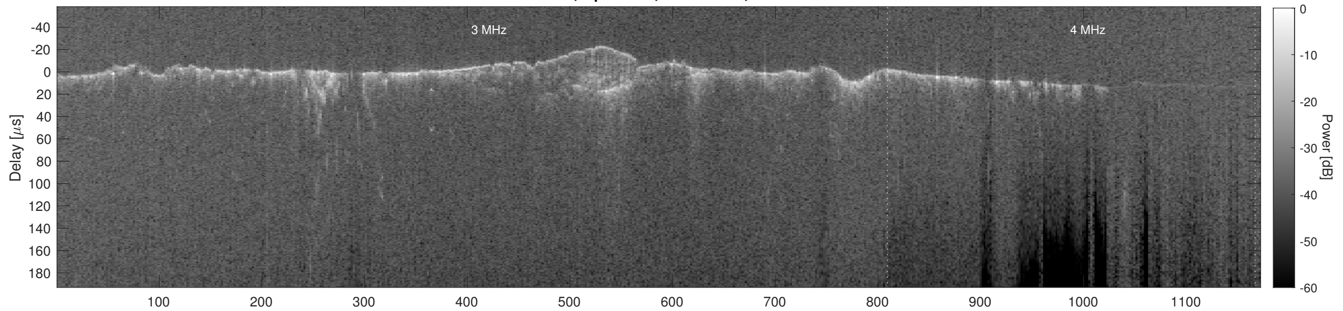
Orbit 12891, Cluttergram
