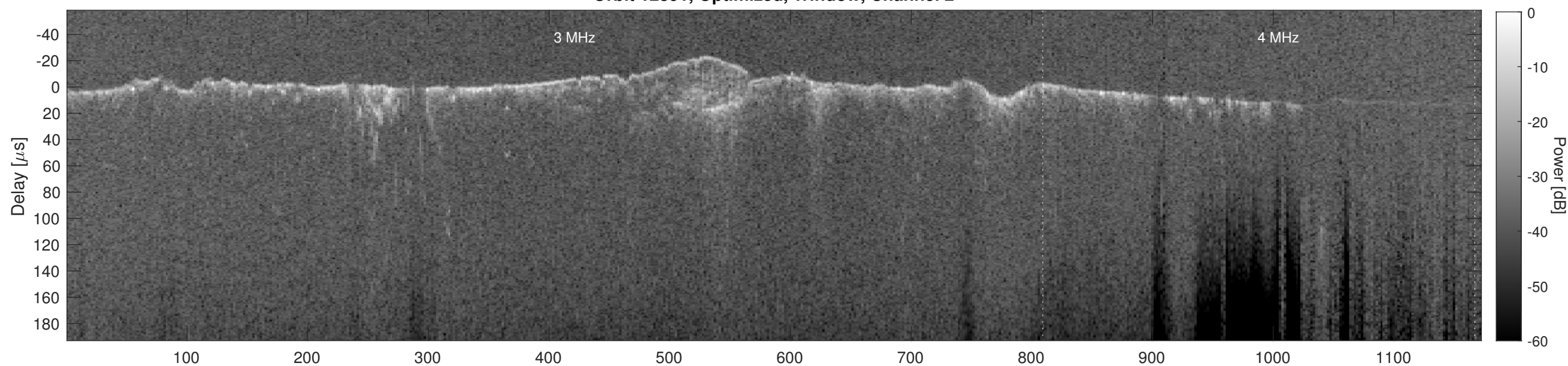
Orbit 12891, Cluttergram
