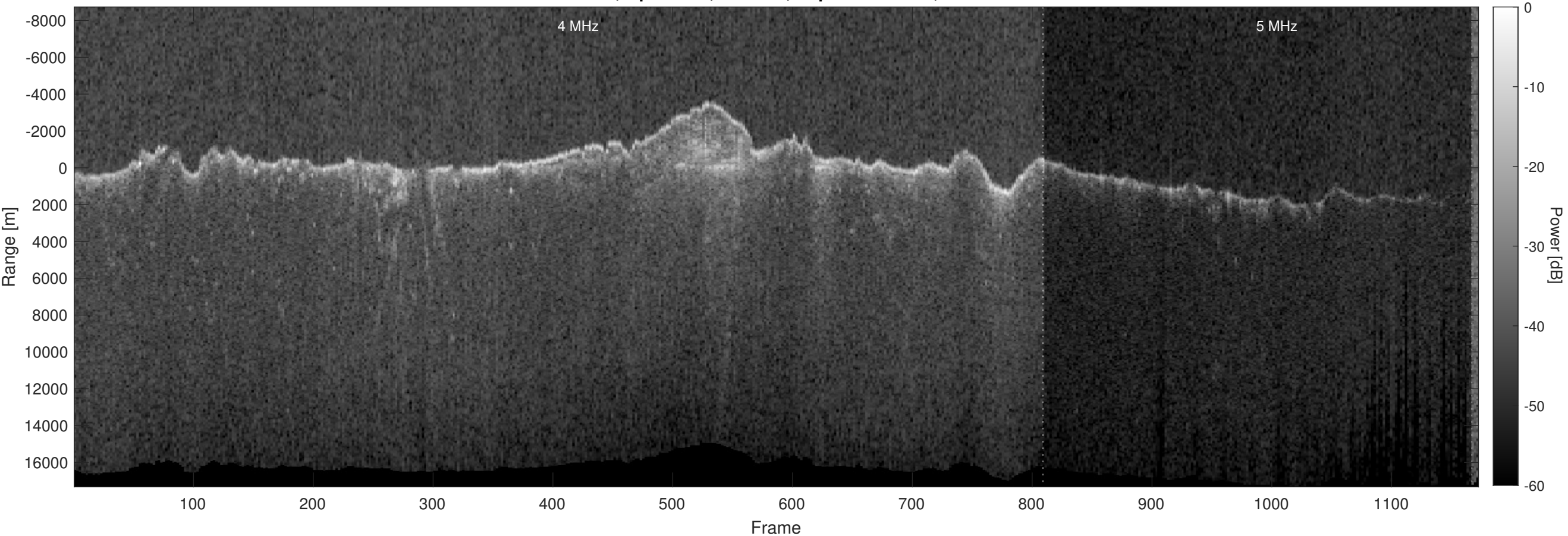
Orbit 12891, Optimized, Window, Depth-Corrected, Channel 2
