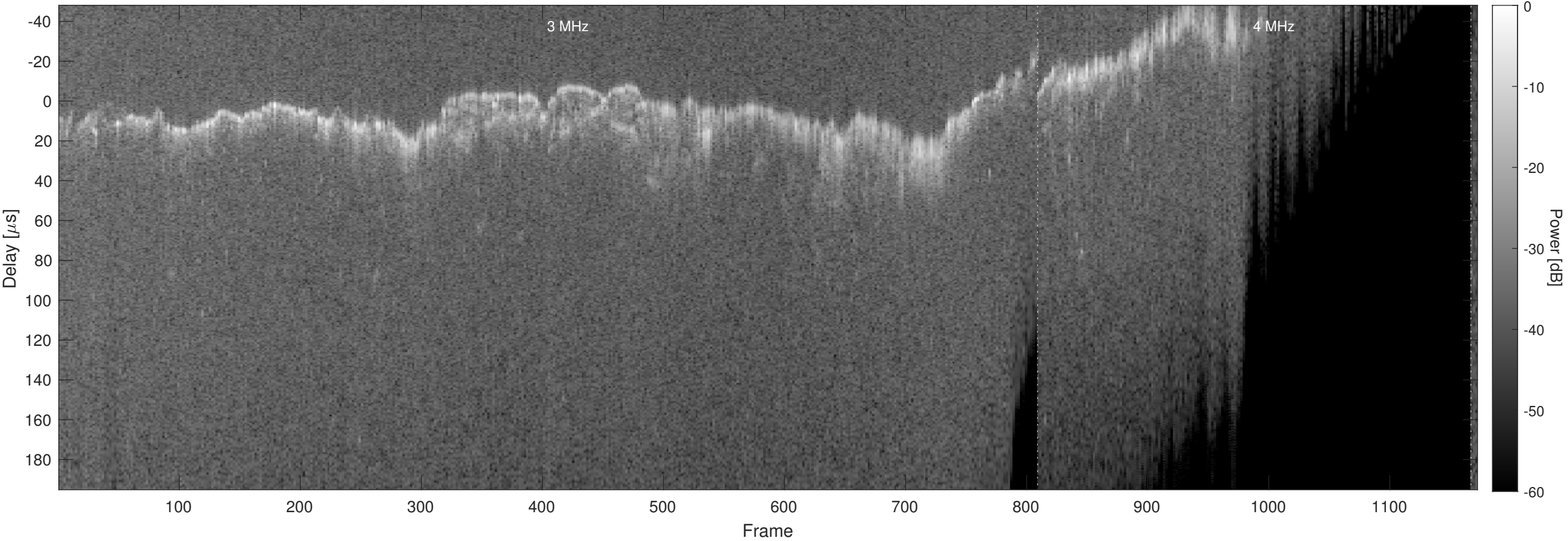
Orbit 12892, Chapman, No Window, Channel 2
