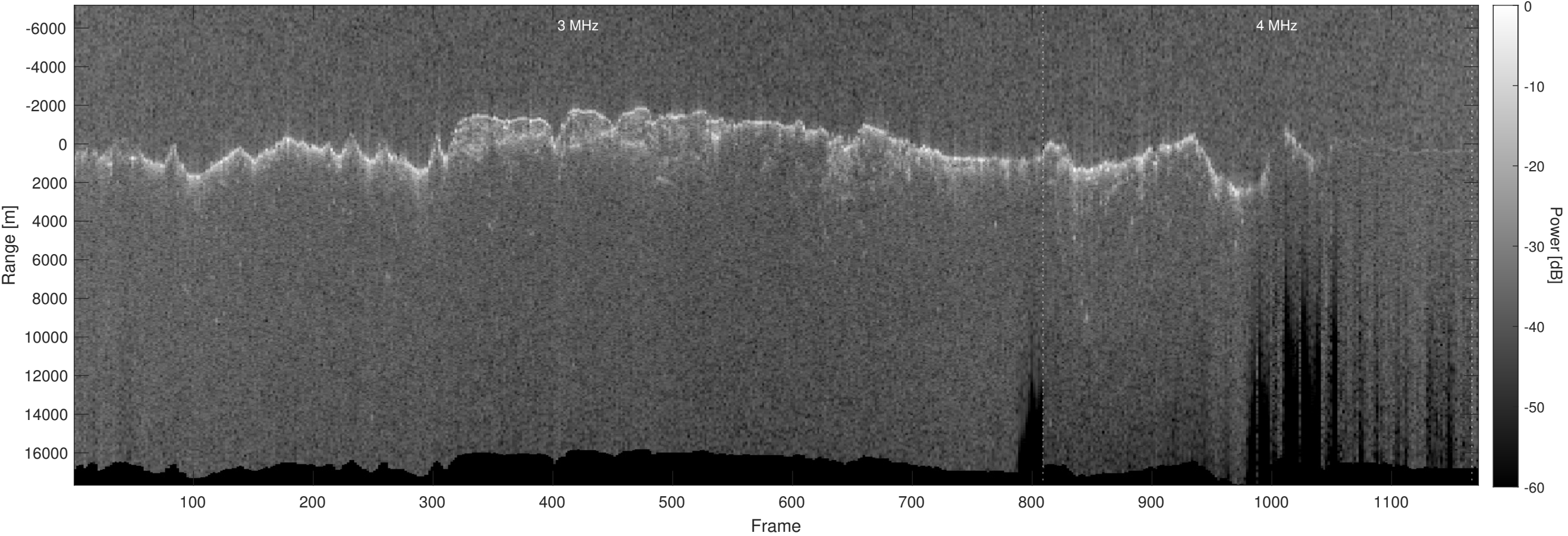
Orbit 12892, Optimized, No Window, Depth-Corrected, Channel 2
