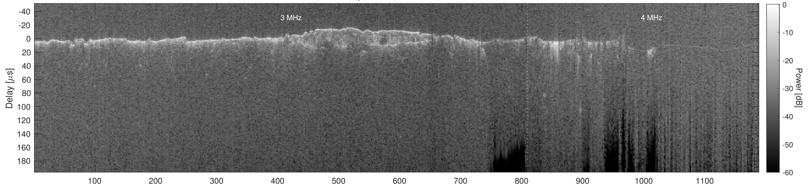
Orbit 12893, Cluttergram
