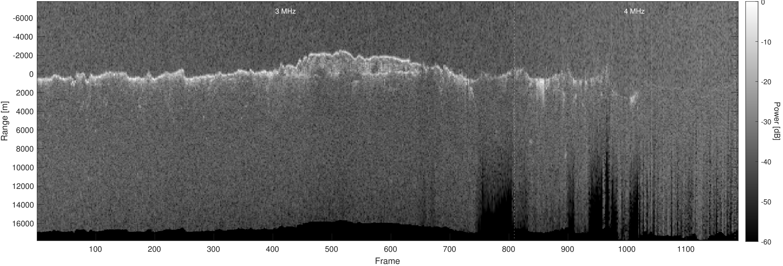
Orbit 12893, Optimized, Window, Depth-Corrected, Channel 2
