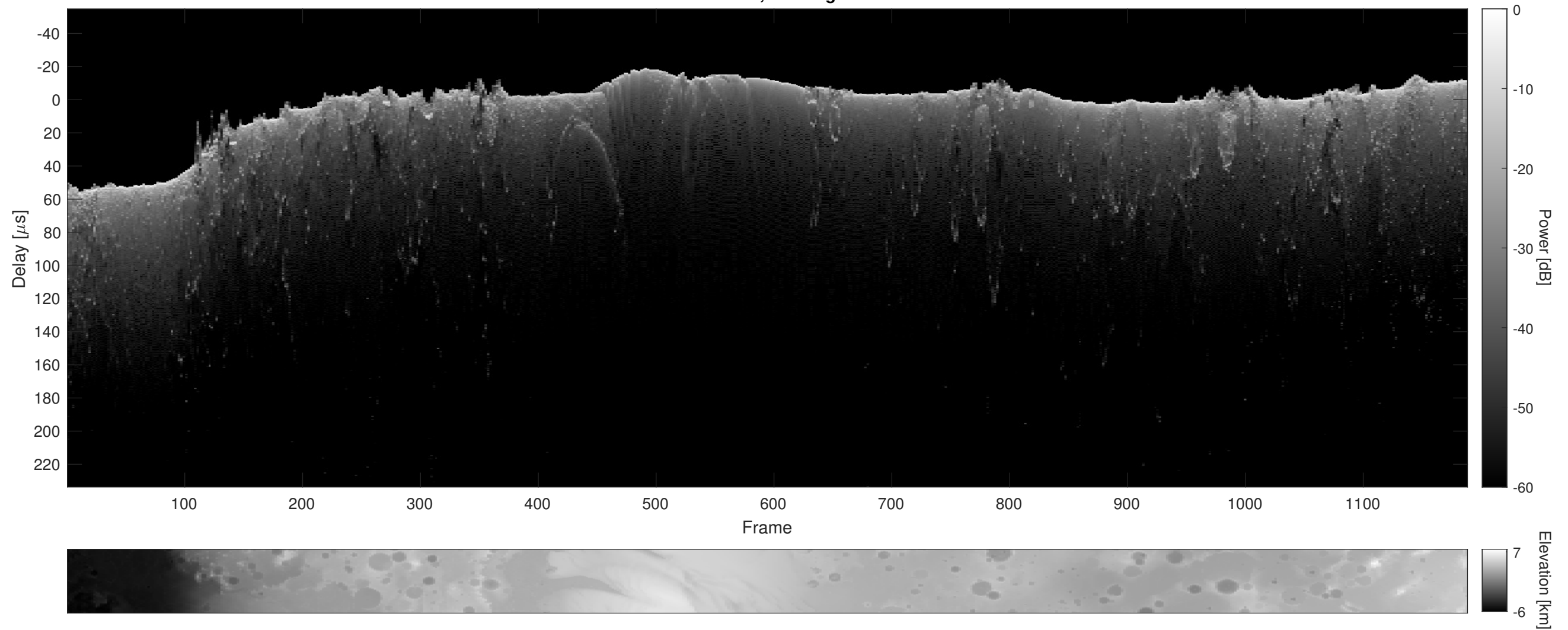
Orbit 12896, Cluttergram
