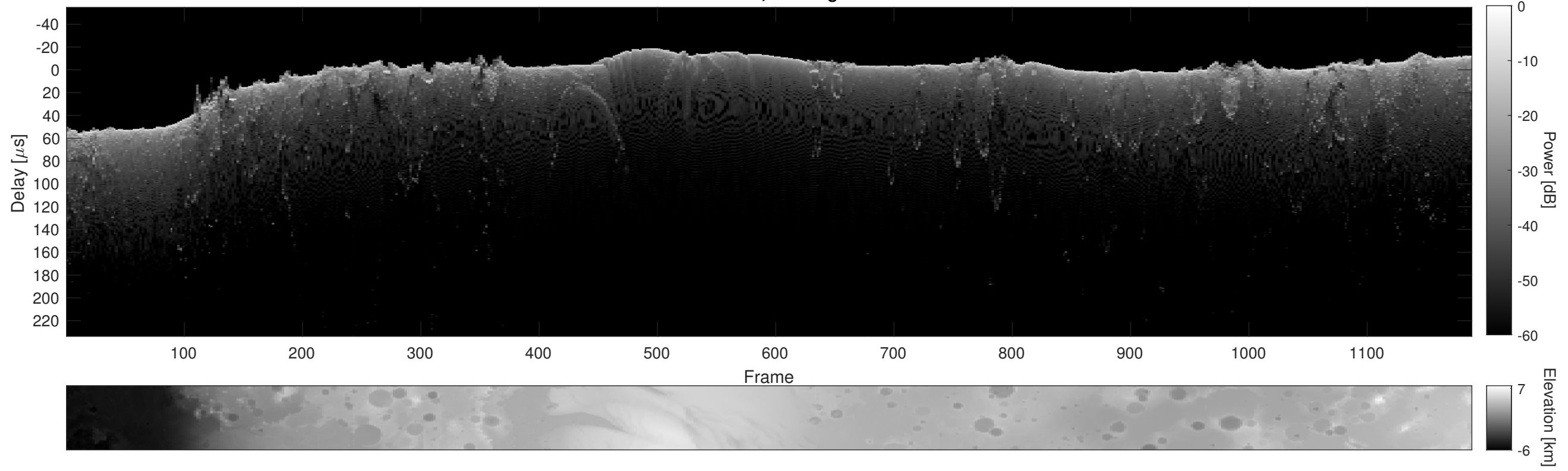
Orbit 12896, Cluttergram
