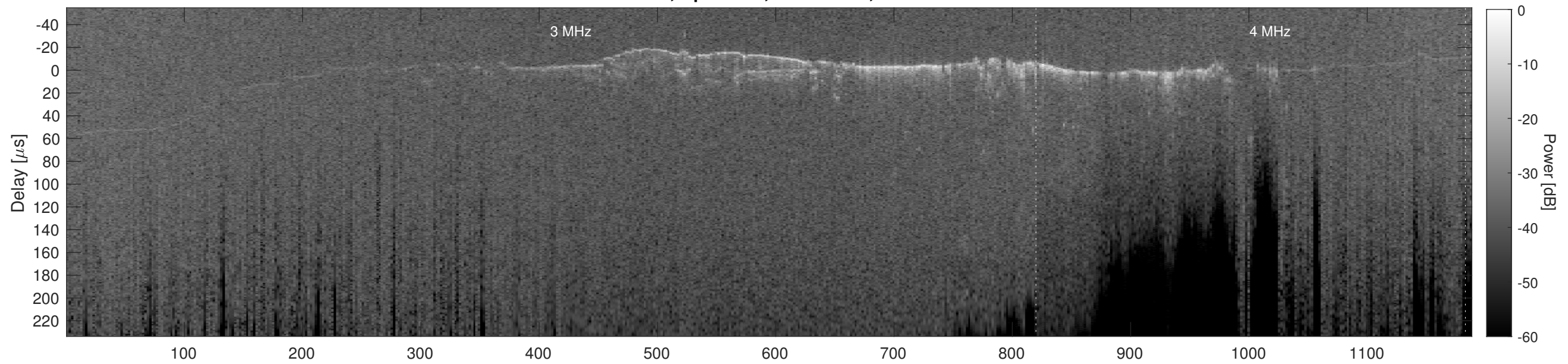
Orbit 12896, Cluttergram
