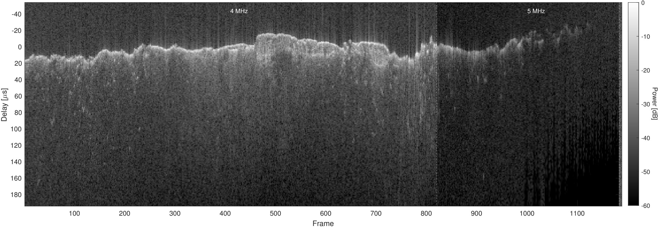
Orbit 12897, Chapman, No Window, Channel 2
