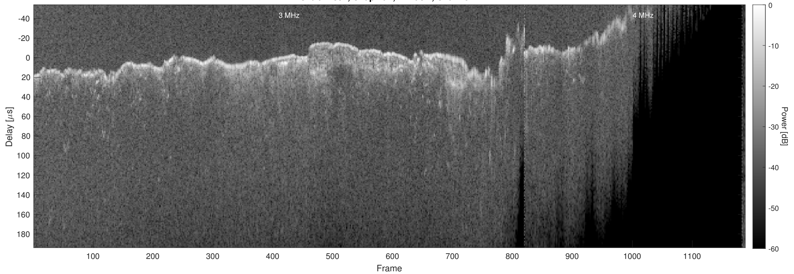
Orbit 12897, Chapman, Window, Channel 2
