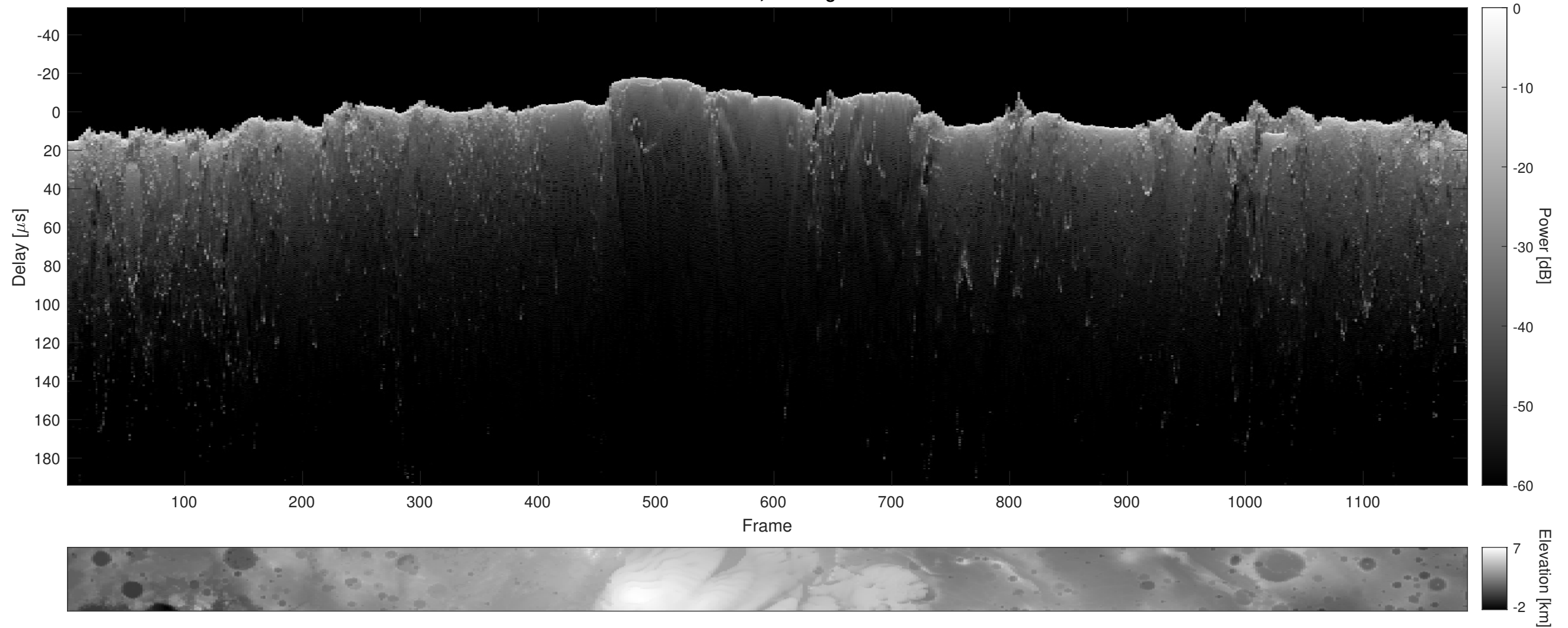
Orbit 12897, Cluttergram
