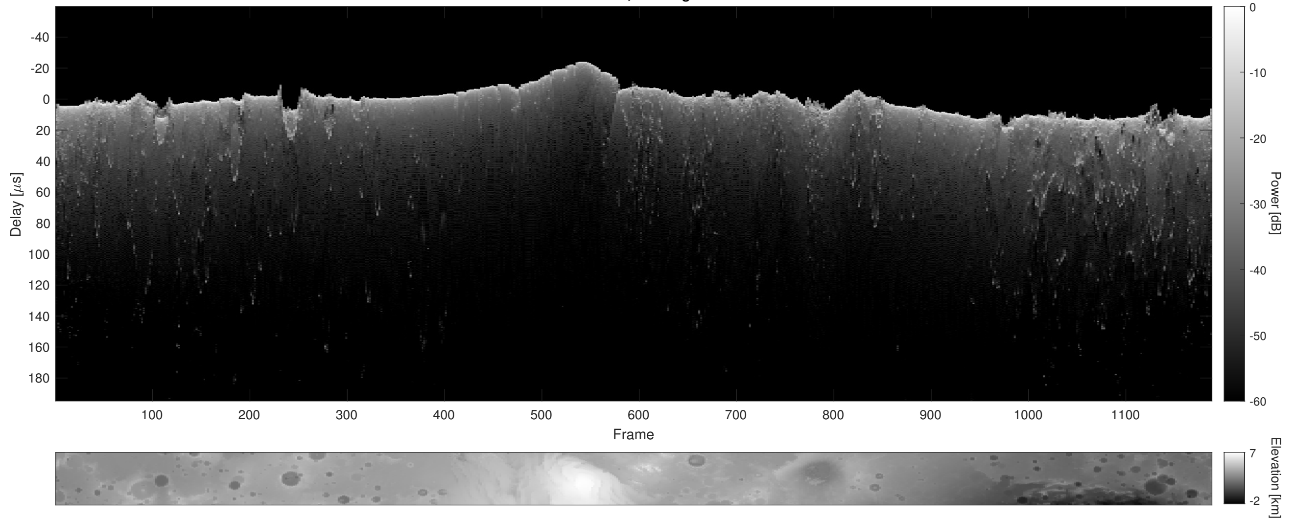
Orbit 12898, Cluttergram
