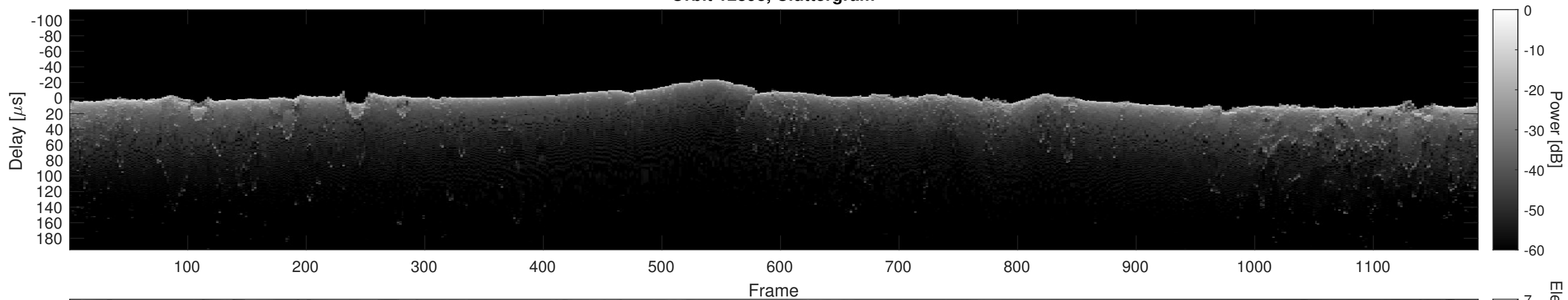
Orbit 12898, Cluttergram
