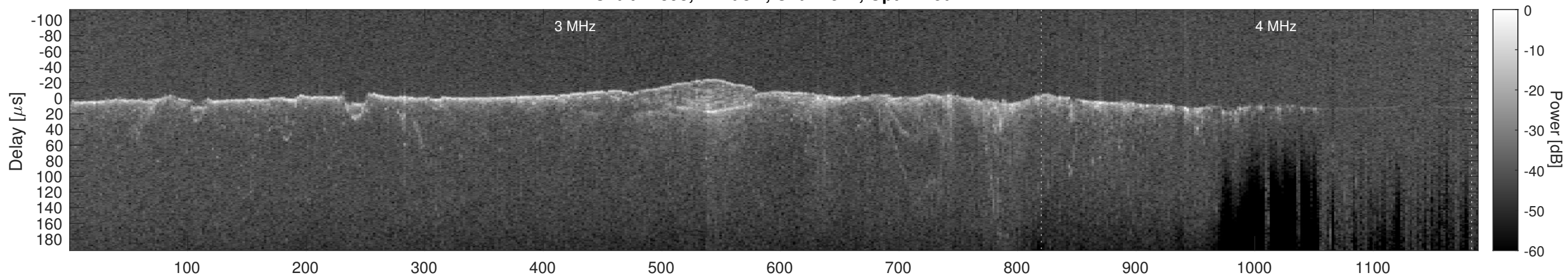
Orbit 12898, Cluttergram
