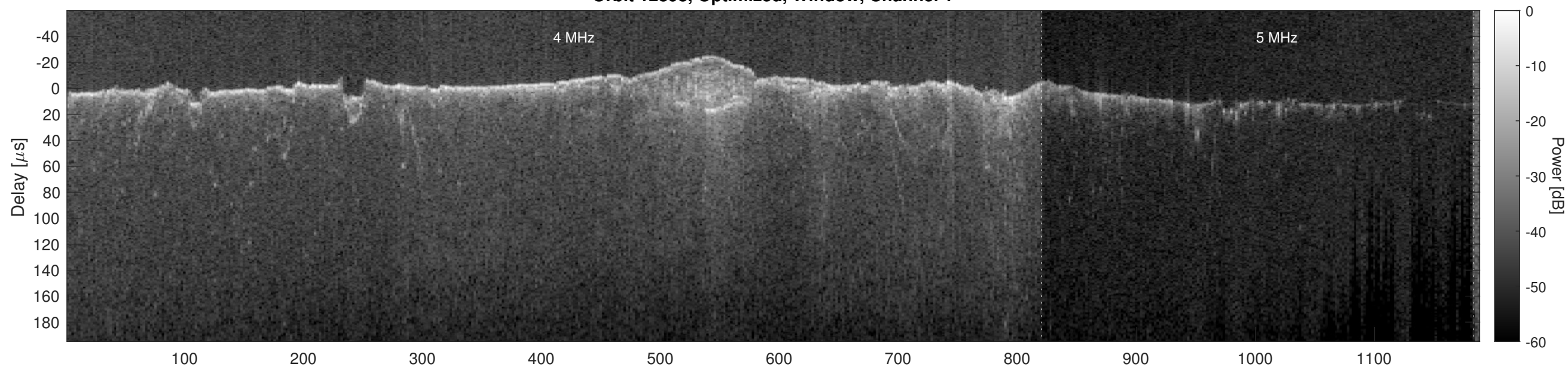
Orbit 12898, Optimized, Window, Channel 2
