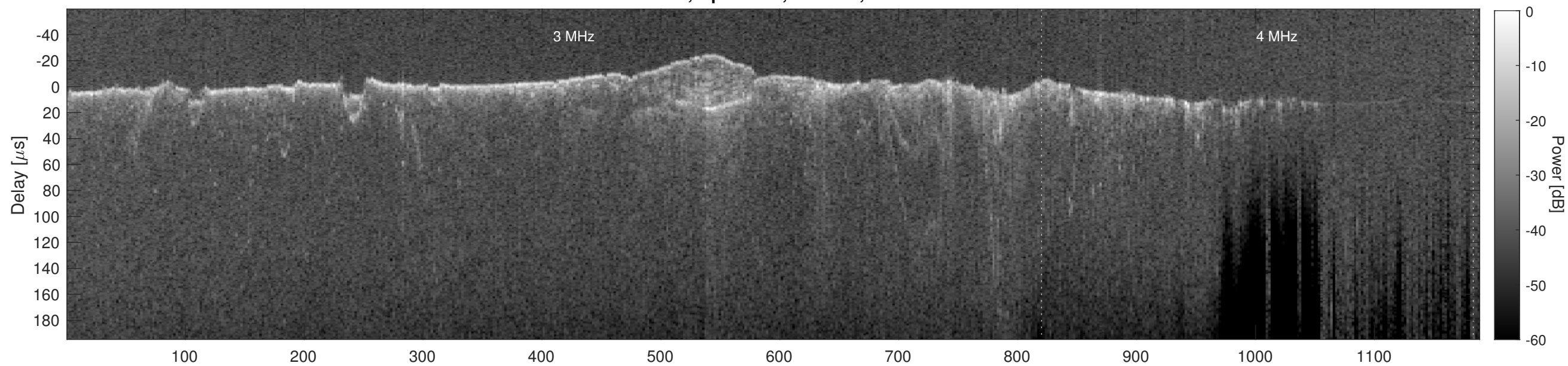
Orbit 12898, Cluttergram
