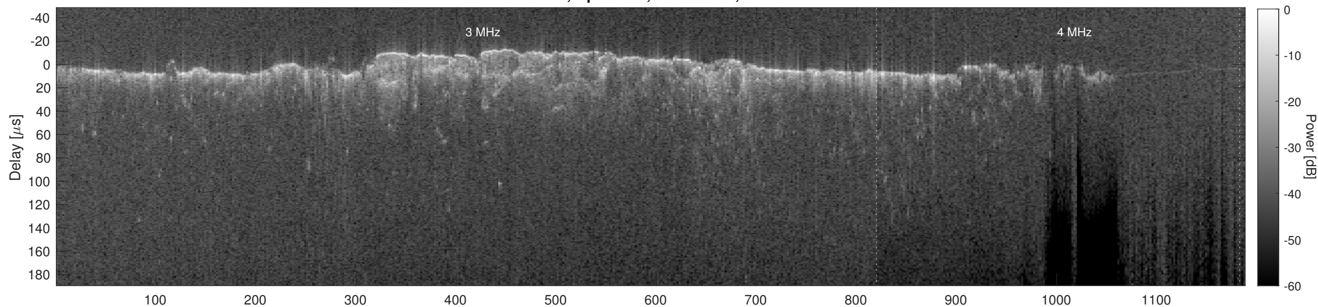
Orbit 12899, Cluttergram
