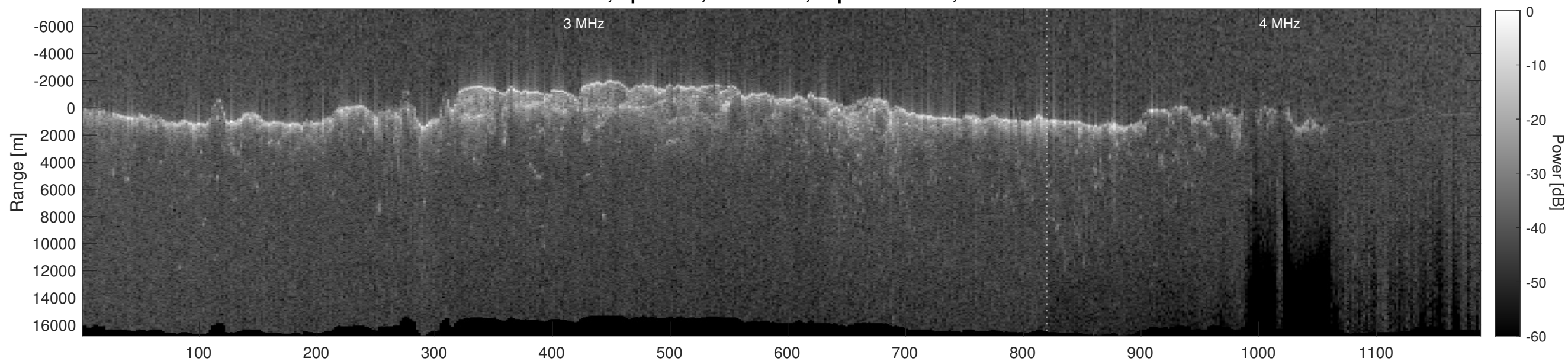
Orbit 12899, Depth-Corrected Cluttergram
