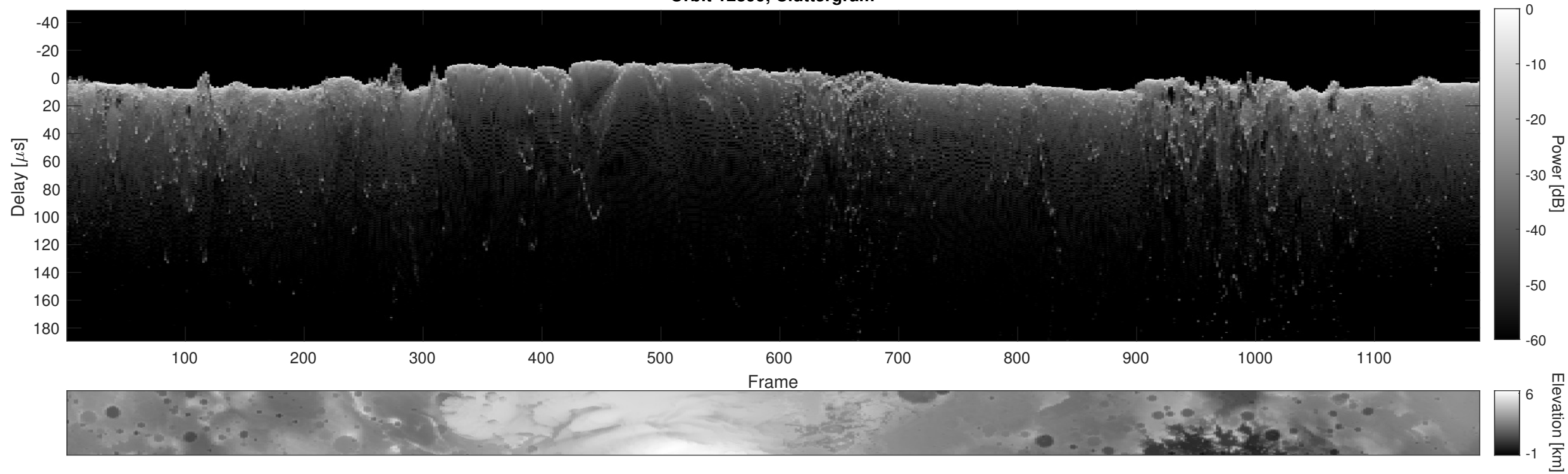
Orbit 12899, Cluttergram
