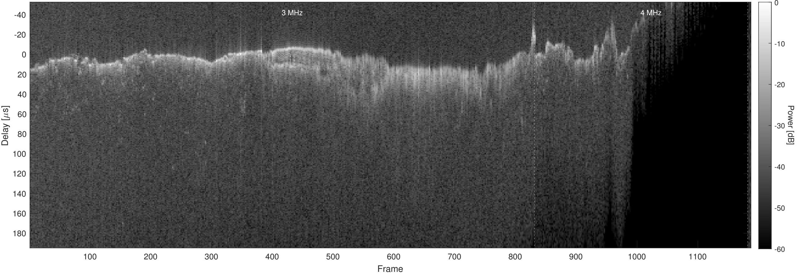
Orbit 12902, Chapman, No Window, Channel 2
