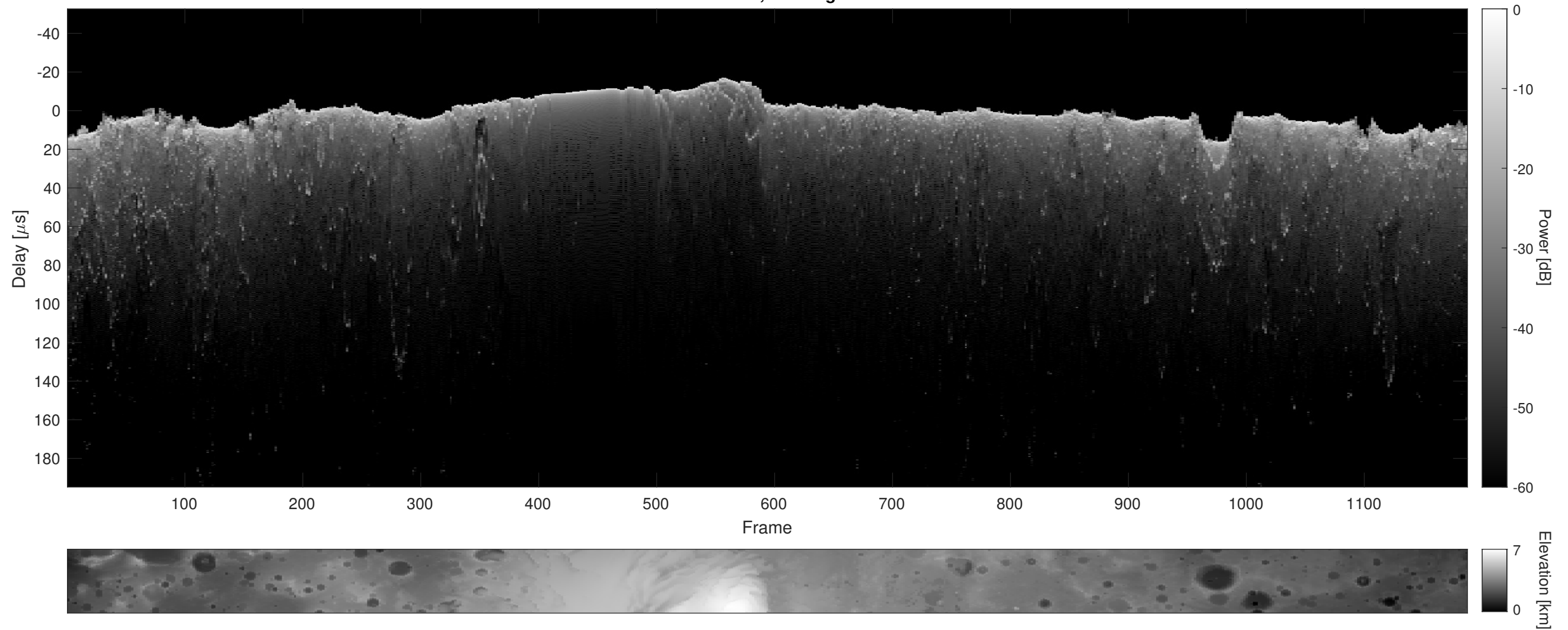
Orbit 12902, Cluttergram
