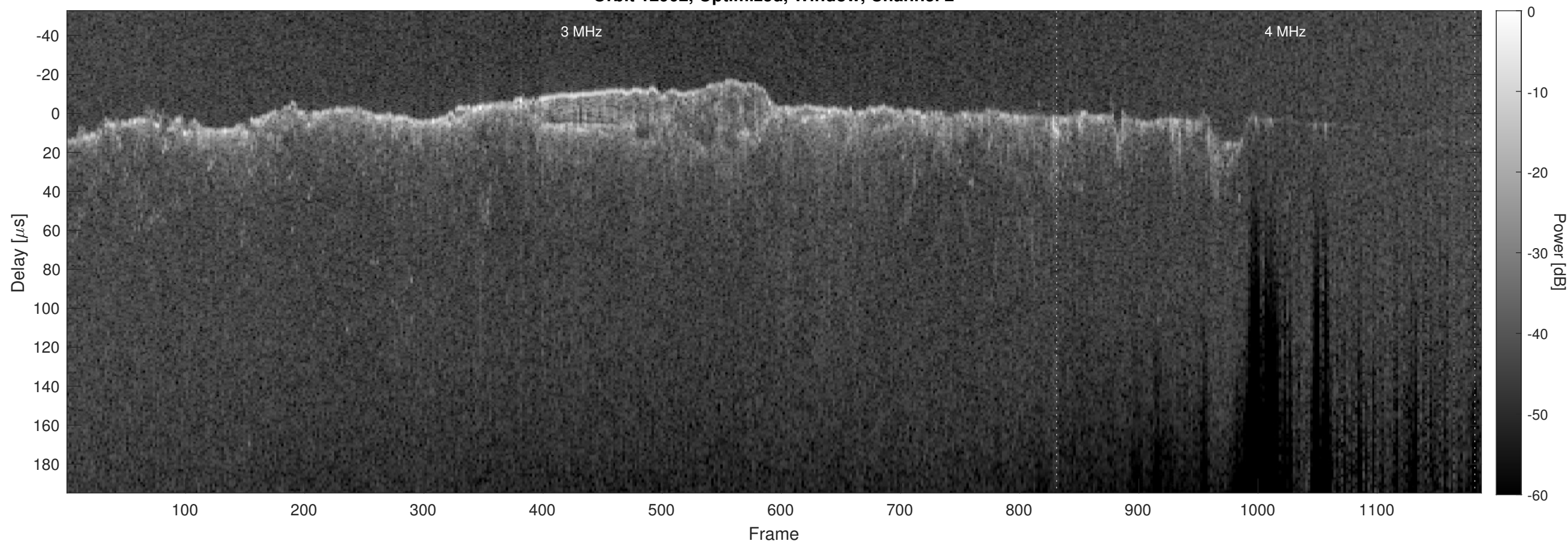
Orbit 12902, Optimized, Window, Channel 2
