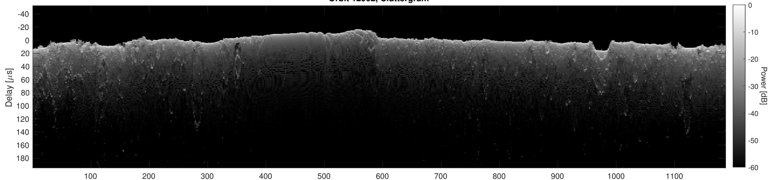
Orbit 12902, Cluttergram
