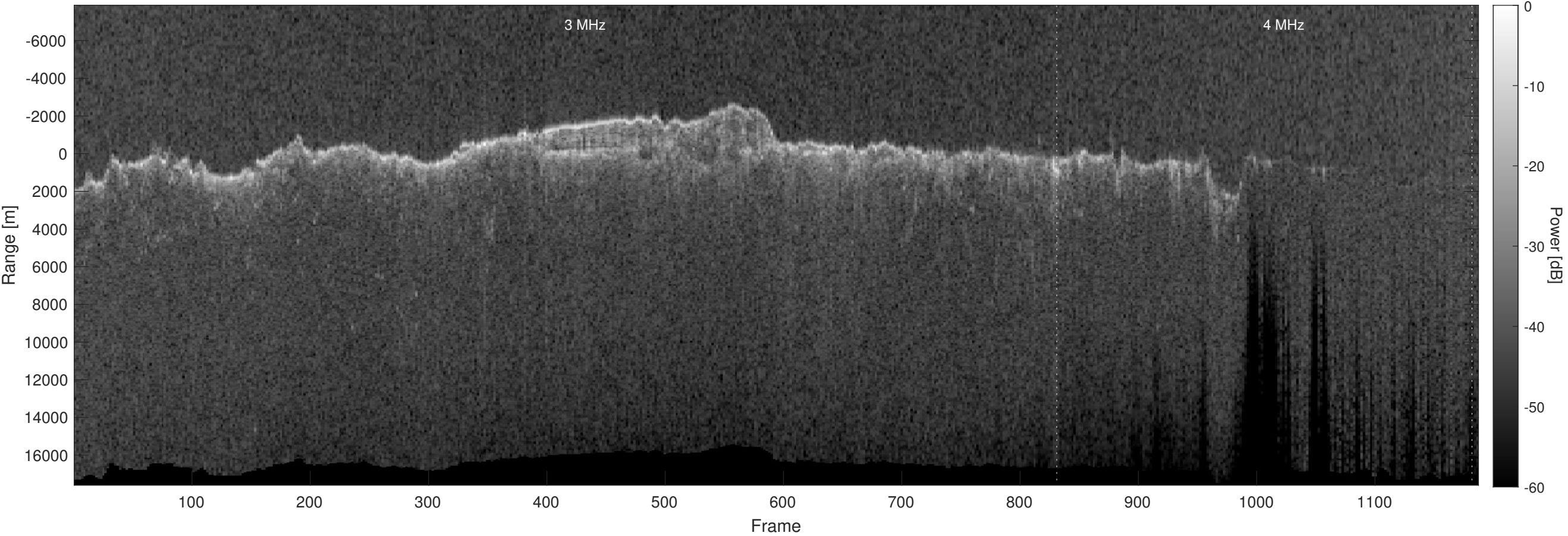
Orbit 12902, Optimized, Window, Depth-Corrected, Channel 2
