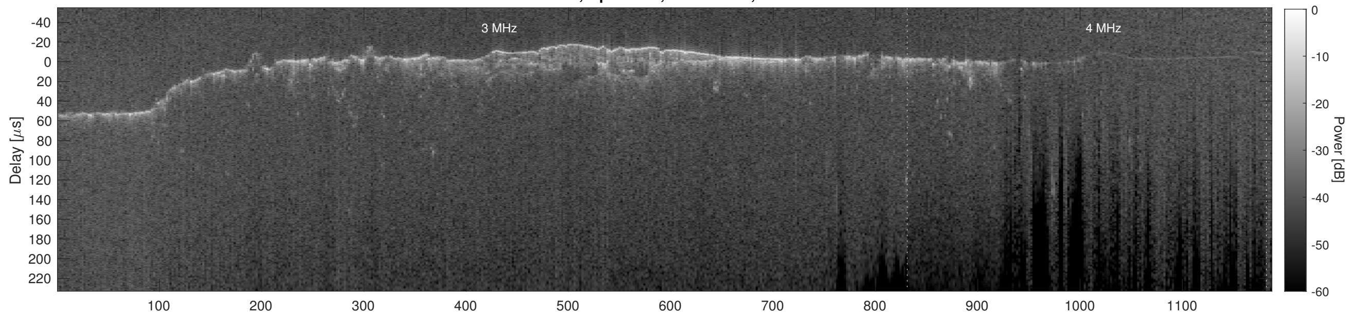
Orbit 12903, Cluttergram
