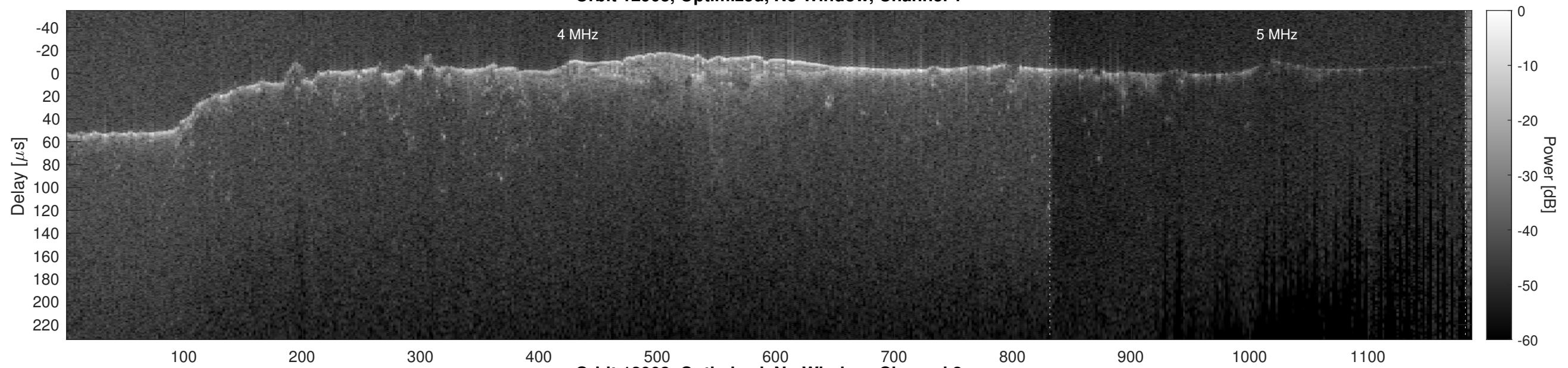
Orbit 12903, Optimized, No Window, Channel 2
